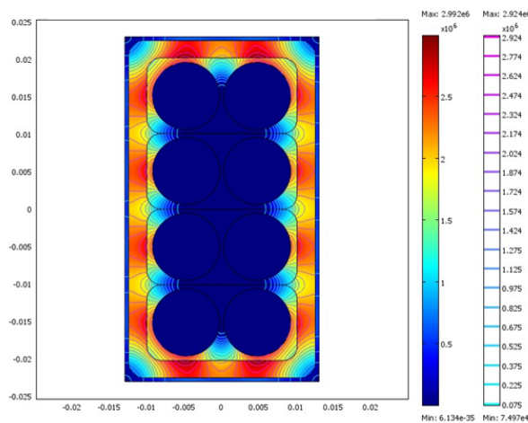
Fig. 4 Electrical field distribution of circular winding (V/m)
