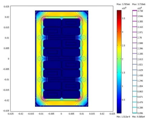
Fig. 2.b Electrical field distribution of rectangular winding (V/m) - direct cooling with water
