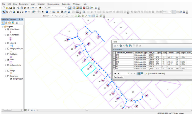
Fig. 1 Storm sewer network with associated drainage table, as viewed in the database
