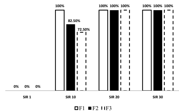
Fig. 19: Relay maloperation for faults at t = 0.205 sec and for different SIR
