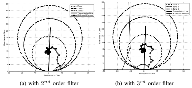
Fig. 17: Impedance loci with 2 nd and 3 rd order filter for R phase to ground fault at t = 0.205 sec and at 100 km ( SIR = 30 , \delta_s = 30 )
