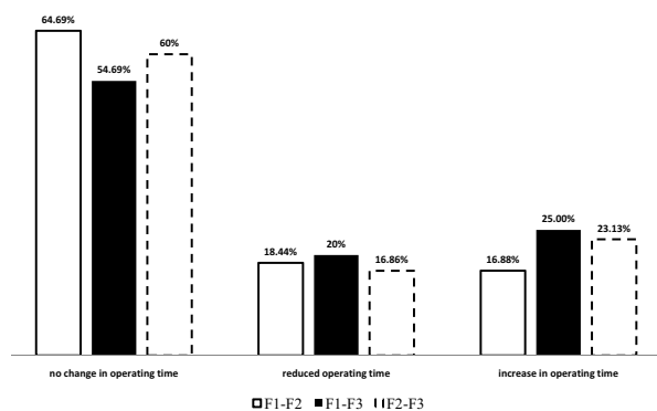
Fig. 8: Comparison of difference in operating time for faults at t = 0.2 sec with 1 st , 2 nd and 3 rd order filters in relay model
