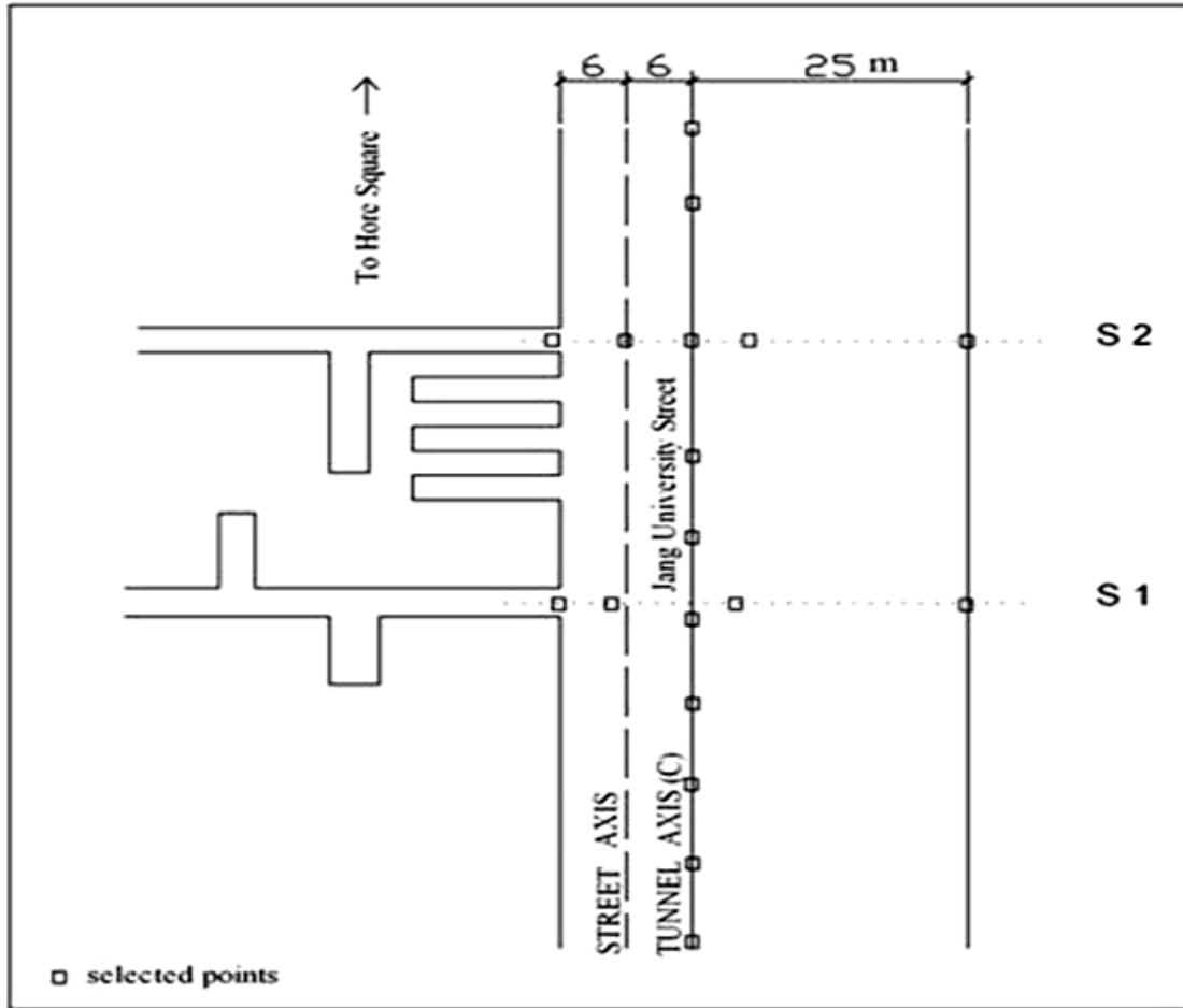
Fig. 1 Locations of points for field measurement
