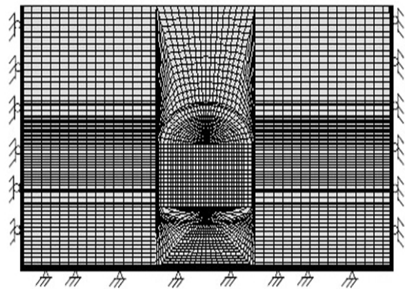
Fig. 3 Mesh used in the analysis of tunnels
