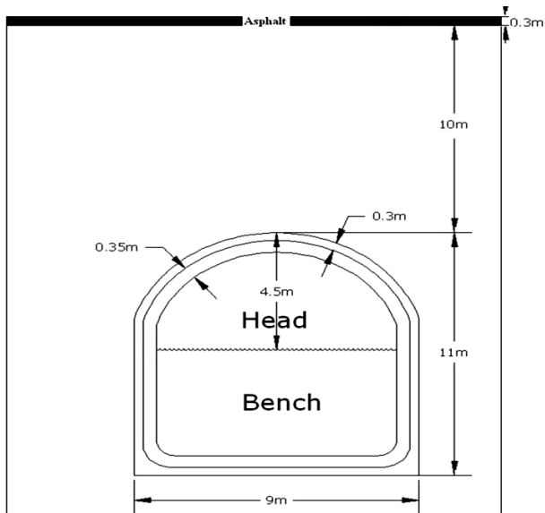
Fig. 2 Tunnel geometry
