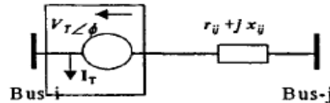
Fig. 2 Equivalent circuit for TCPST
