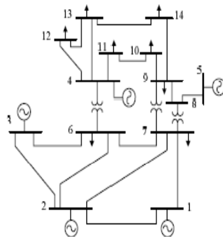
Fig. 4 Single line diagram for IEEE 14 Bus system
