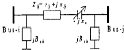
Fig. 1 Model of TCSC
