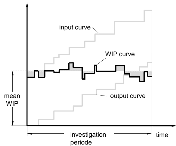
Fig. 6 Throughput Diagram including WIP curve
