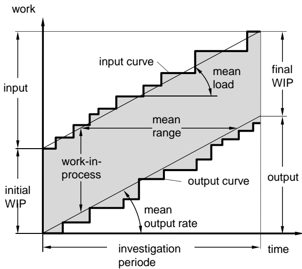
Fig. 5 Throughput Diagram
