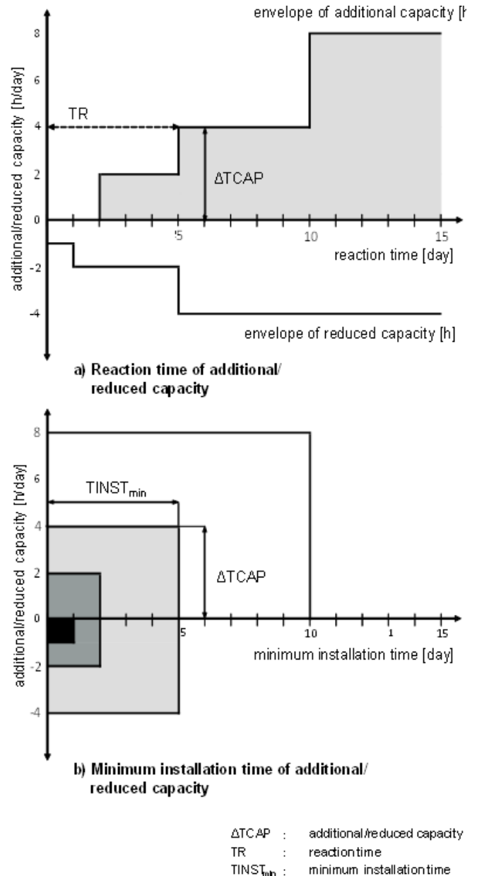
Fig. 2 Capacity envelope
