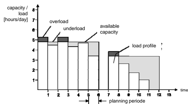
Fig. 1 Capacity graph
