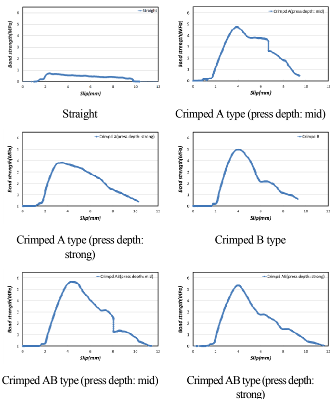
Fig. 9 Slip-bond strength curves per test variable
