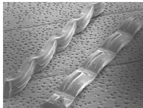
Crimped B type (heat treated during deformation)
