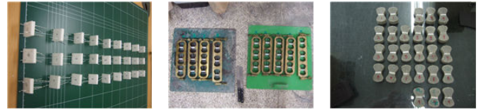
Fig. 7 Fabrication process of specimens
