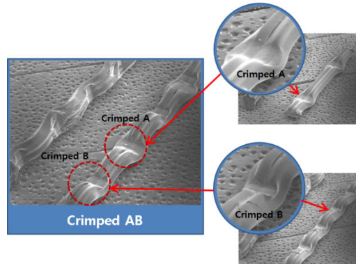
Fig. 5 Hybrid crimping of the developed PP fiber
