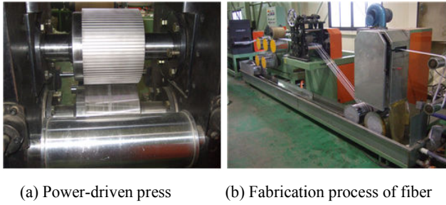
Fig. 2 Press casting process of fiber
