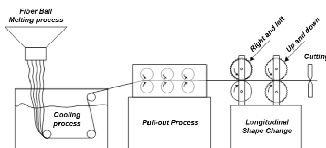
Fig. 1 Schematic fabrication process of the developed fiber
