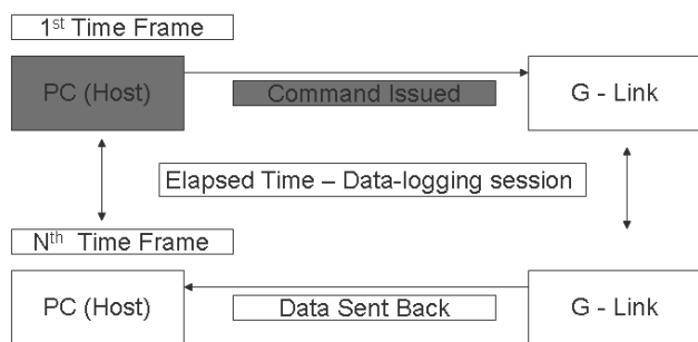
Fig. 4 Flow of data during a trigger session
