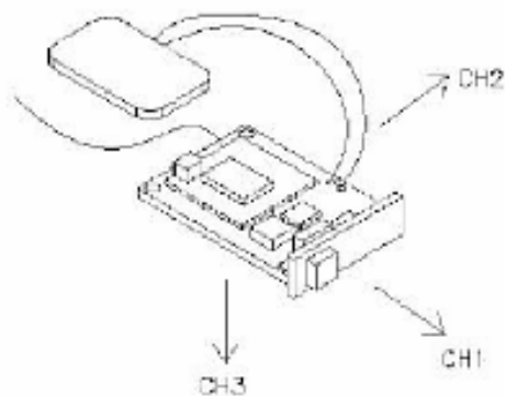
Fig. 1 The Triaxial Accelerometer
