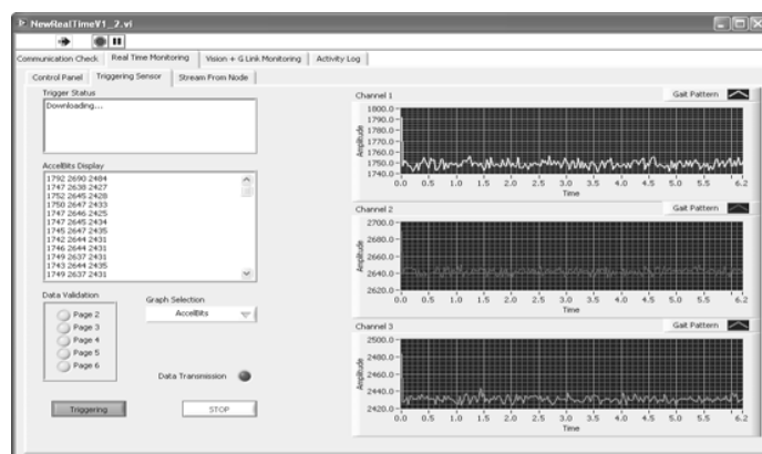
Fig. 6 Data Acquisition Panel
