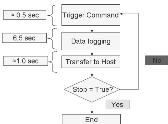
Fig. 5 Process flow for capturing data
