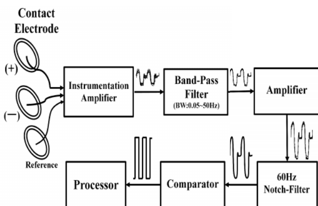
Fig. 2 Measurement circuit of EOG signal
