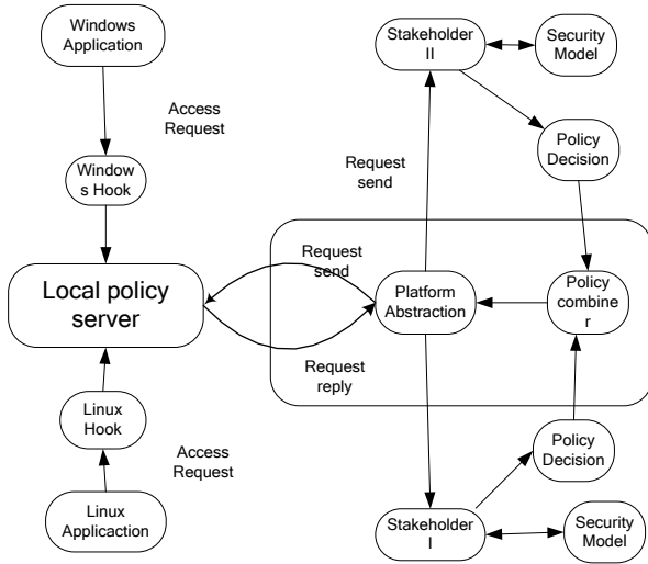
Fig. 1 Overview of the framework
