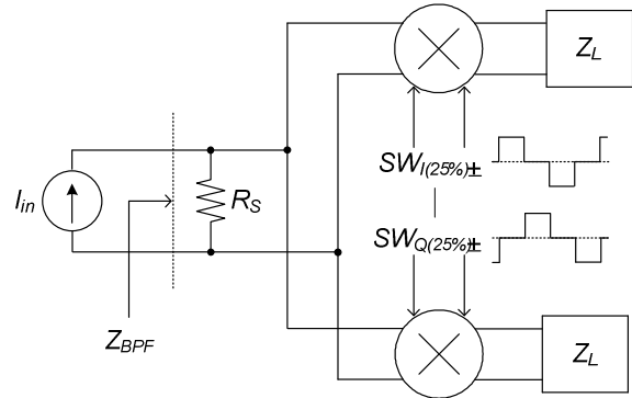
Fig. 3 A tunable impedance Z_{in-IQ} with image cancellation
