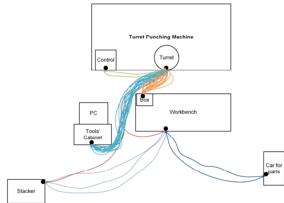
Fig. 4 Spaghetti chart (initial situation)
