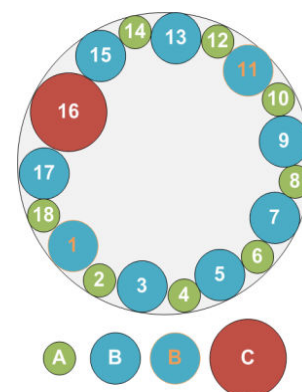
Fig. 2 Layout of the punching machine's turret
