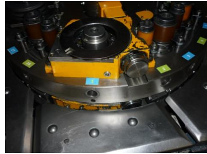
Fig. 6 Identification of positions in the turret
