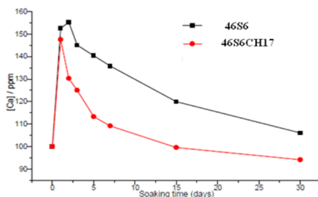
Fig. 1 Evolution of elemental concentrations of Ca in SBF solution measured by ICP-OES, versus soaking times
