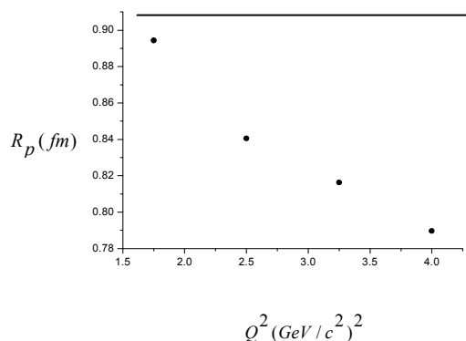
Fig. 2 The bag radius neutron vs of Q^2
