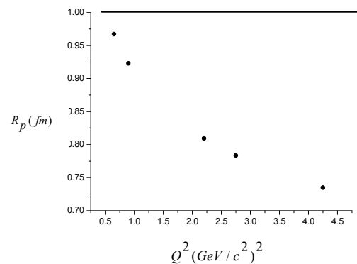
Fig. 1 The bag radius proton vs of Q^2
