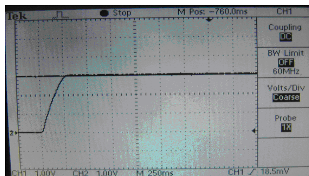
Fig. 17 Response of VRP fuzzy controller with range of 0.049 volt
