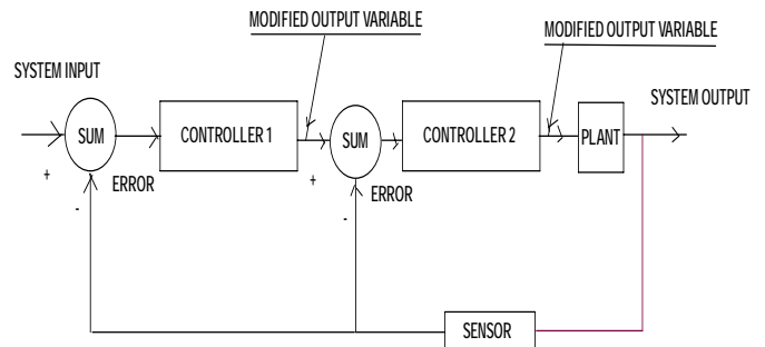
Fig. 9 Proposed Fuzzy Logic Controller with Variable Reference
