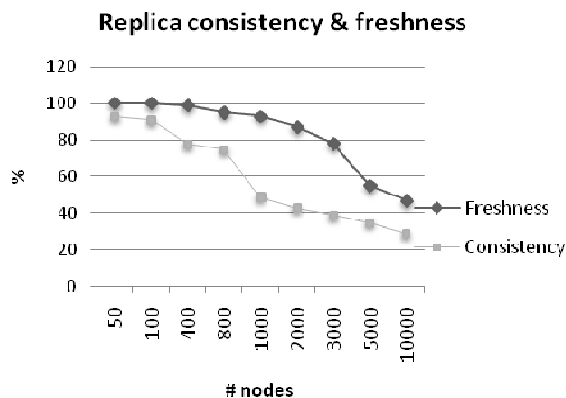
Fig. 7 Consistency& Freshness
