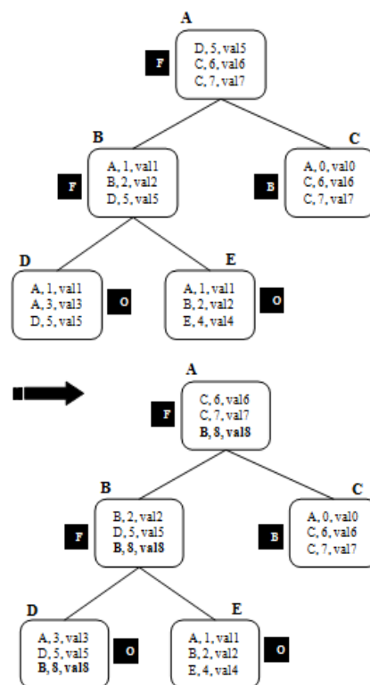
Fig. 4 Write example
