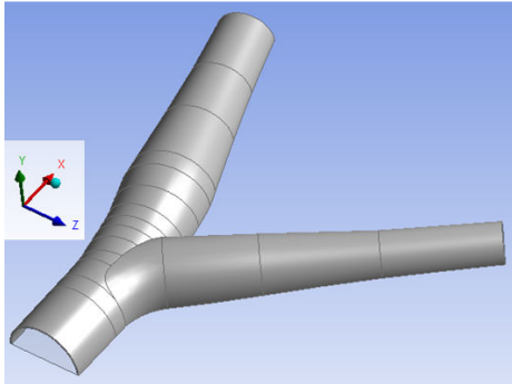
Fig. 1 The carotid artery geometry with arterial thickness
