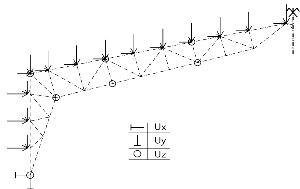
Fig. 4 Scheme of specified boundary conditions – supports, loads
