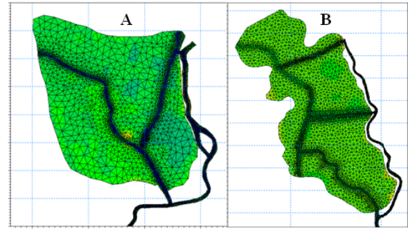
Fig. 6 Cell size of the cohesive sediment transport model for BK (A) and EBK (B)
