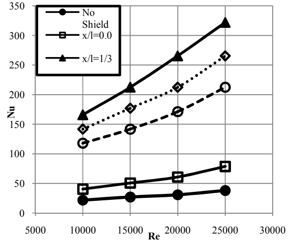
Fig. 8 Nusselt numbers versus Reynolds numbers at different shield positions
