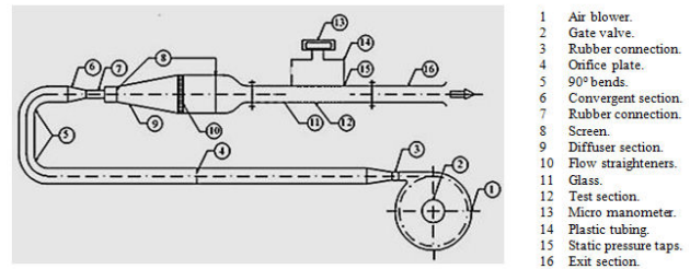
Fig. 1 Schematic diagram of test rig and instrumentation
