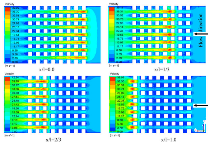
Fig. 5 Velocity distribution at y = 0.01 m at various shield positions for Re = 25000
