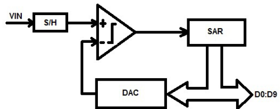
Fig. 1 SAR ADC architecture
