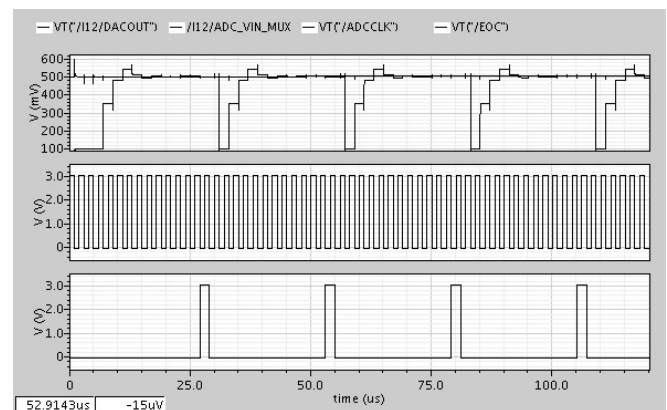
Fig. 12 DAC simulation
