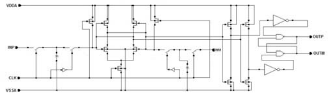
Fig. 7 Dynamic latch
