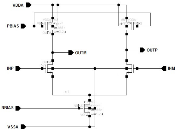
Fig. 4 Single-stage fully differential amplifier
