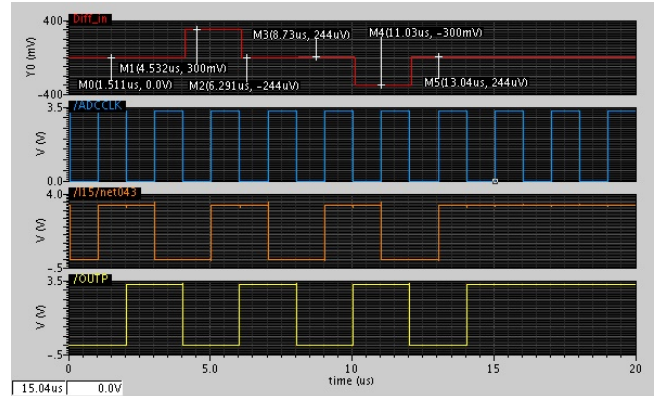
Fig. 10 Comparator result
