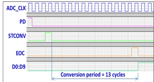
Fig. 11 SAR logic timing diagram
