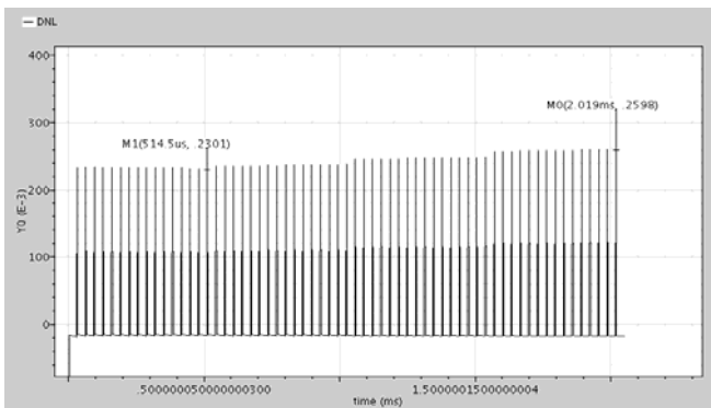
Fig. 9 Simulated DNL
