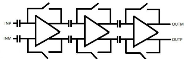
Fig. 6 Pre-amplifier with a noise cancellation circuit
