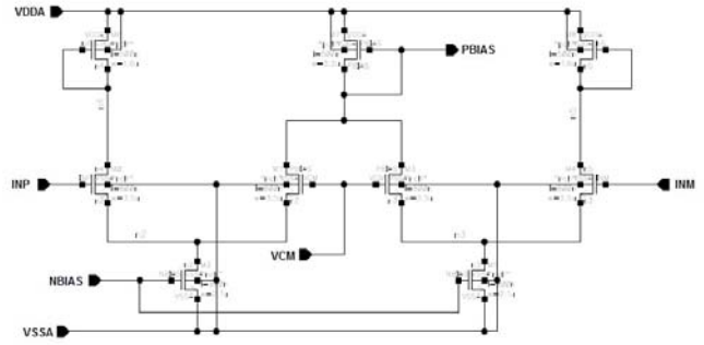
Fig. 5 Common mode feedback circuit
