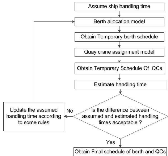
Fig. 6 Flow chart of functional integration with feed back
