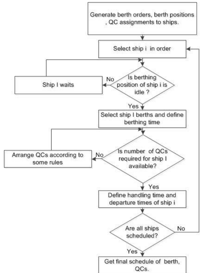
Fig. 7 Flow chart of simultaneous integration
