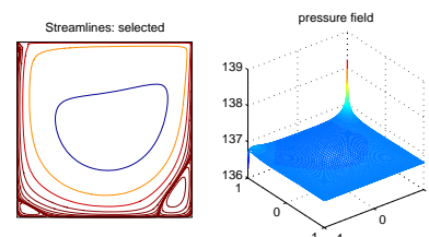
Fig. 2. Navier - Stokes flow solution plot(steady cavity problem, Q2-P1, 128 × 128 stretched grids, \nu = 0.001 ). Left: streamline plot. Right: pressure plot.
