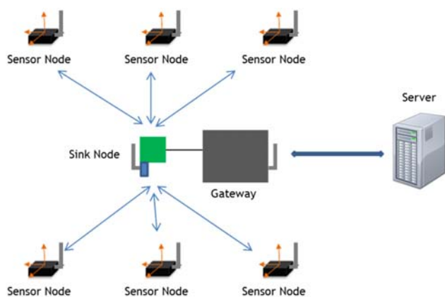
Fig. 1 Configuration of the car parking monitoring system
