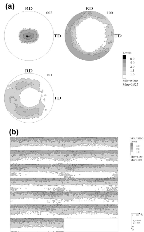
Fig. 3 The complete pole figures (a) and ODF (b) of specimen produced by warm rolling
