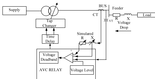
Fig. 2 AVC relay scheme with LDC
