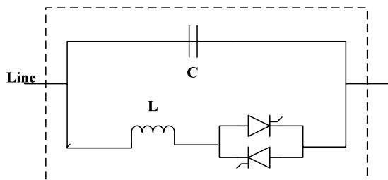
Fig. 5 Thyristor-Controlled Series Compensation
