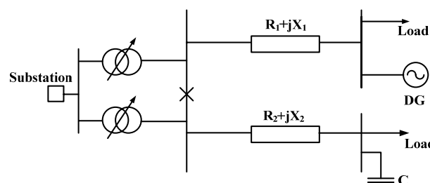
Fig. 1 Simple system for voltage control
