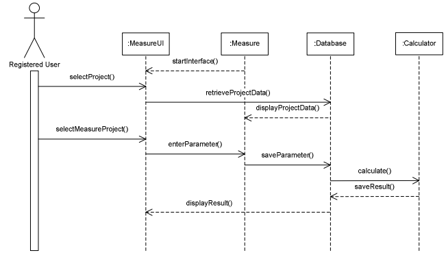
Fig. 10 Sequence diagram for measure project
