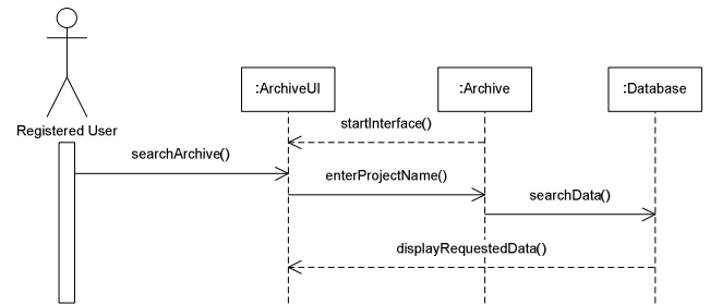
Fig. 11 Sequence diagram for search archive
