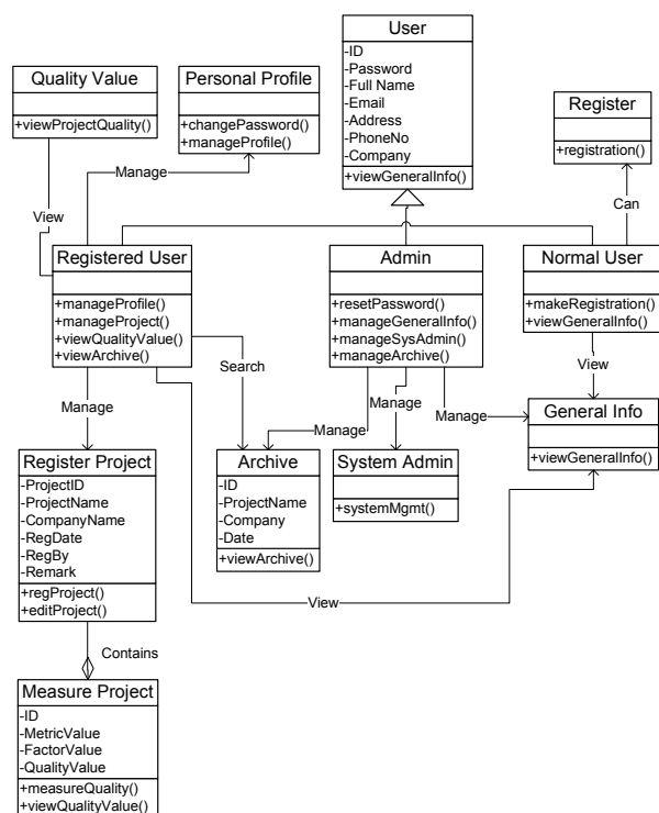
Fig. 4 Class Diagram
