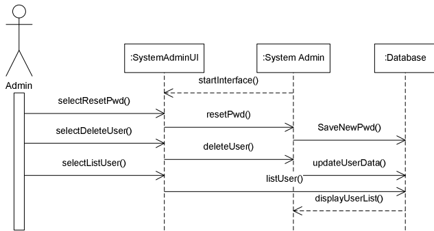
Fig. 7 Sequence diagram for system admin
