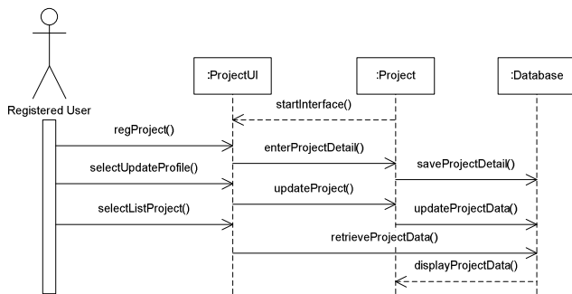
Fig. 9 Sequence diagram for register project
