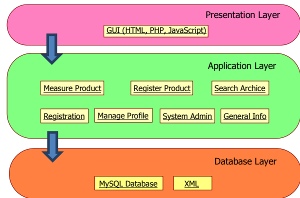
Fig. 3 Layered Architecture
