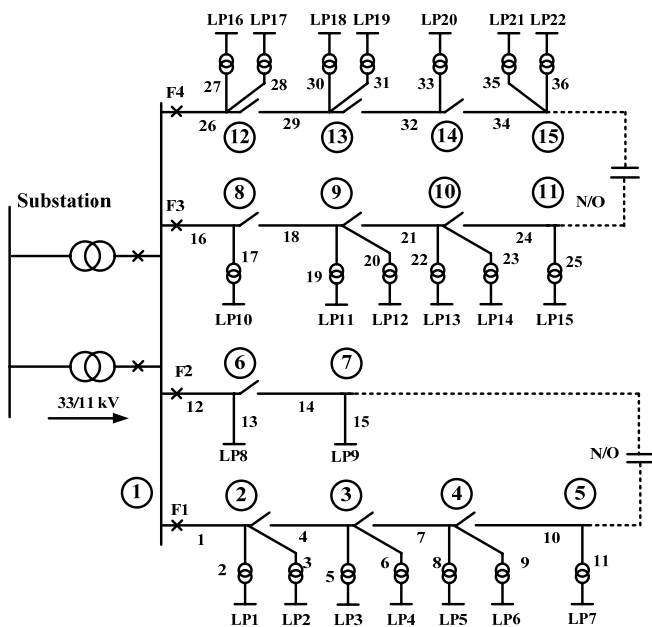
Fig. 4 RBTS bus 2 Radial Distribution system
