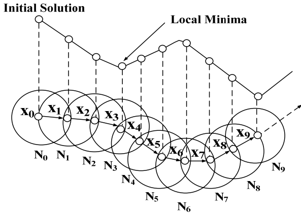
Fig. 1 Search direction of Tabu search
