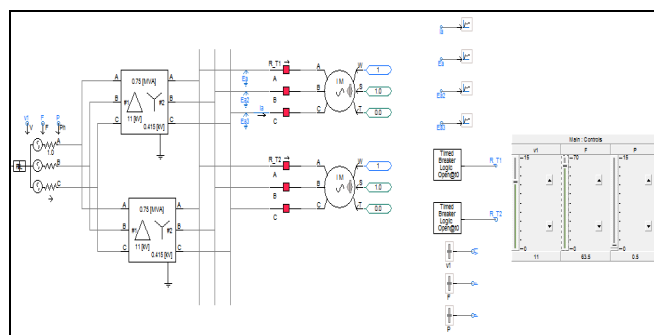
Fig. 1 Simple Large Induction Motor Starting at Substation No.5
