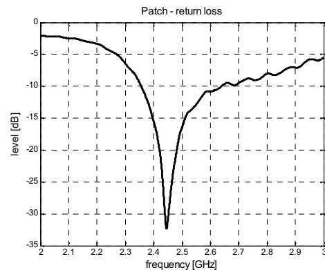
Fig. 6 Patch – return loss
