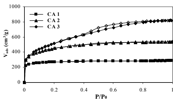
Fig. 1 Adsorption-desorption isotherms of N_2 on activated carbons
