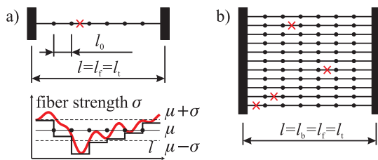
Fig. 3. Unidirectional fibrous structures with breaks at peak load: a) one fiber discretized into segments of length l_0 with a sketch of a strength random field and its minima; b) Daniels's bundle of (discretized) fibers.
