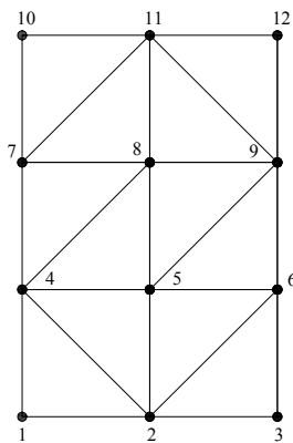
Fig. 6 Graph model of truss G_4 .
