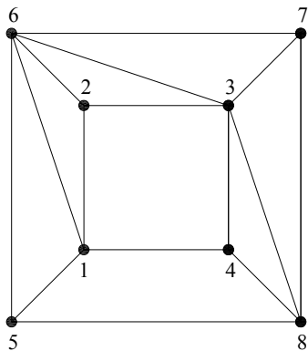
Fig. 5 Graph model of truss G_3 .
