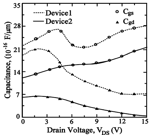
Fig. 8 Capacitance variation for Device1 and Device2
