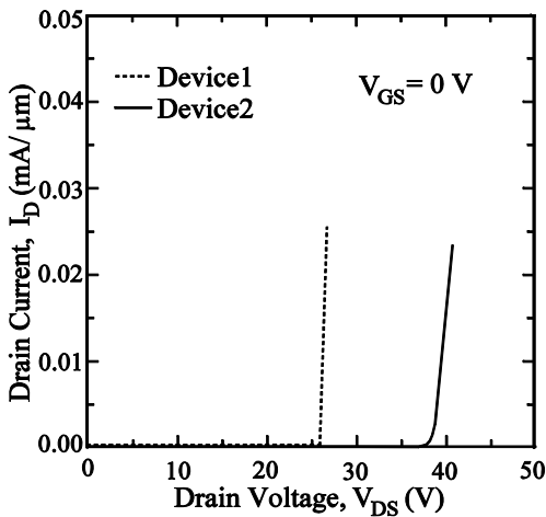
Fig. 5 Breakdown characteristics of Device1 and Device2
