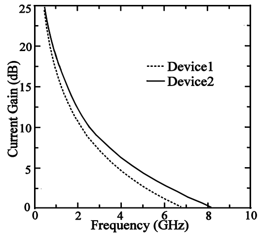
Fig. 7 Frequency response of Device1 and Device2
