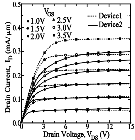
Fig. 2 On-state characteristics of Device1 and Device2
