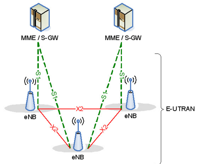
Fig. 1 General architecture of LTE-Advanced system
