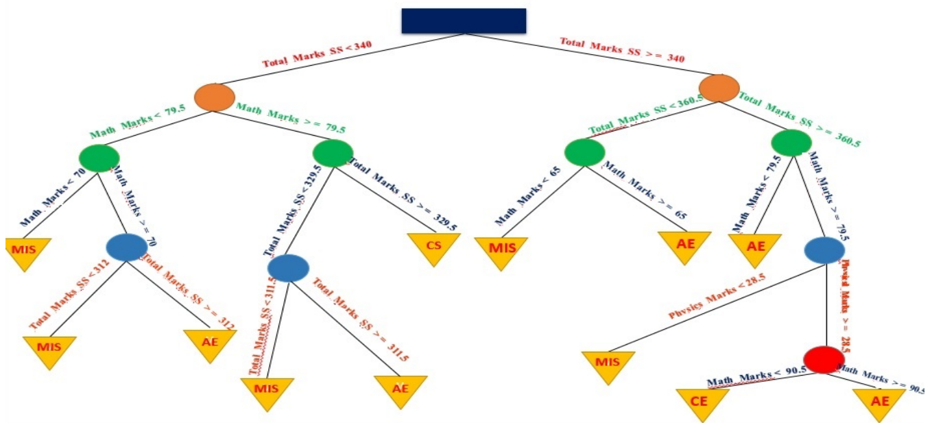
Fig. 2 Decision Tree
