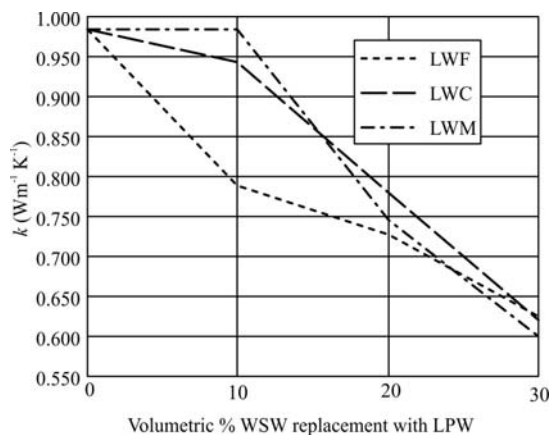
Fig. 1 Relationship between thermal conductivity and WSW amount
