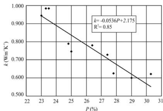
Fig. 3 Relationship between the thermal conductivity and porosity
