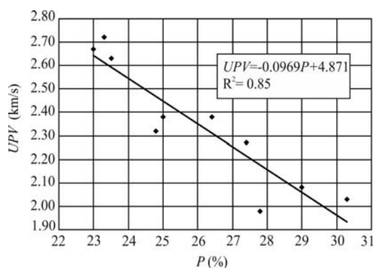
Fig. 4 Relationship between the UPV and porosity
