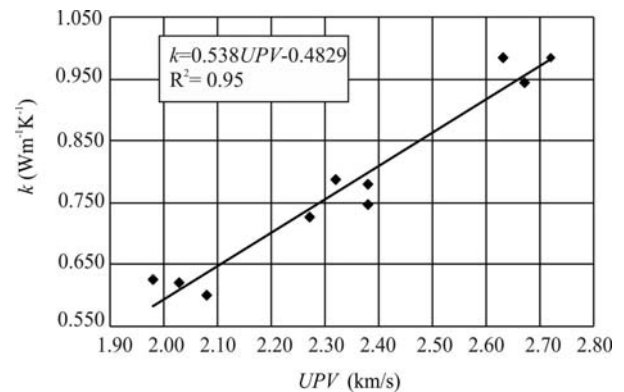
Fig. 2 Relationship between the thermal conductivity and UPV
