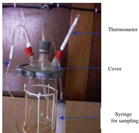
Fig. 2 Bioreactor of fermentation
