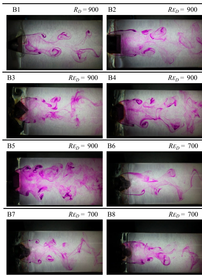
Fig. 9 Vortex formation mechanism for bluff bodies
