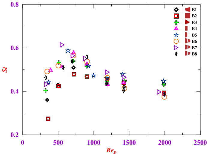
Fig. 4 Variation of Strouhal number with Reynolds number
