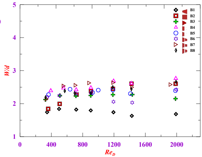
Fig. 6 Variation of wake width with Reynolds number
