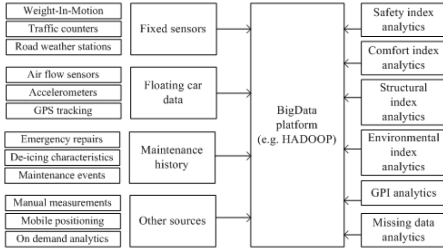
Fig. 2 PeMS configuration for road network [11], [17]
