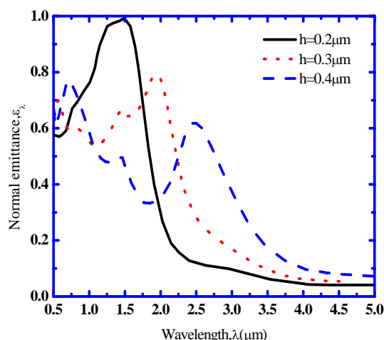
Fig. 4 (Color online) Normal emittance with different grating height, \Lambda = 0.5 \mu\text{m} and f = 0.8 , when TM is perpendicular to the grooves
