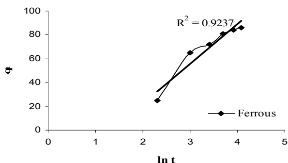
Fig. 11 (a) Elovich kinetic model for ferrous ion adsorption onto Pongamia pinnata bark
