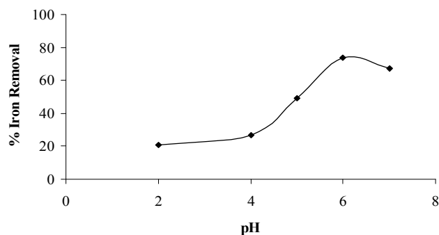
Fig. 13 Effect of pH on adsorption of iron from industrial effluent onto Pongamia pinnata bark
