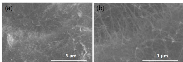
Fig. 5 SEM images of the MCNT film prepared by electrophoretic deposition (EPD) of MCNTs on a graphite tip substrate and heated after emission.
