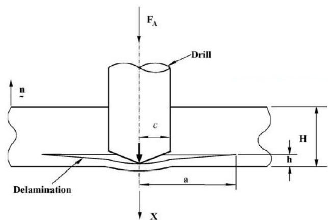
Fig. 1 Delamination zone [4]
