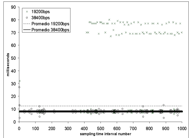
Fig. 2 Sampling time at 19.2 and 38.4 Kbps
