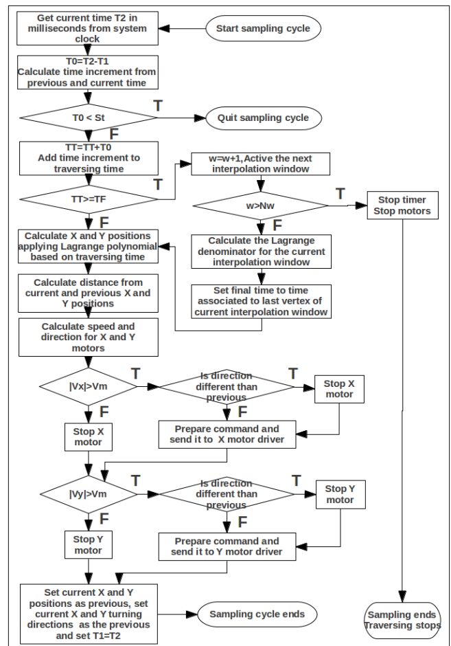
Fig. 3 Command generation flow diagram
