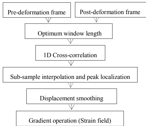
Fig. 4 Axial displacement and strain estimation diagram
