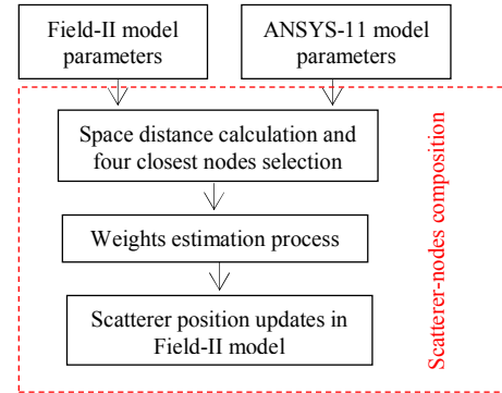
Fig. 2 Scatterer-nodes composition algorithm flowchart
