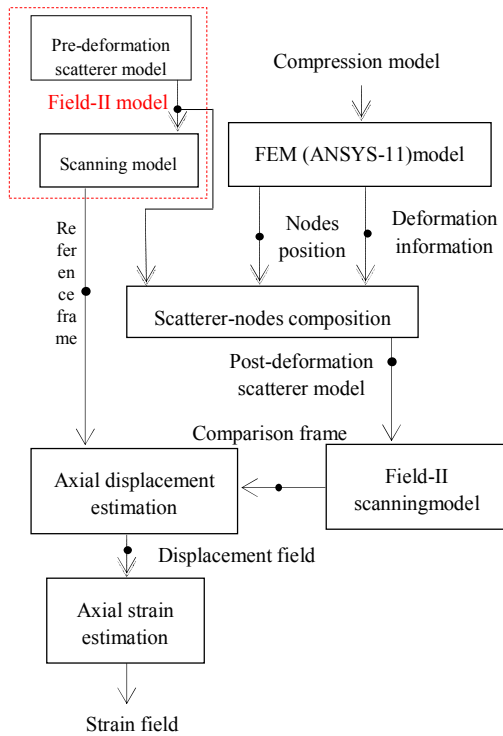
Fig. 1 Block diagram of proposed methodology
