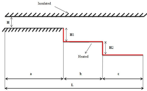
Fig. 1 Geometry domain
