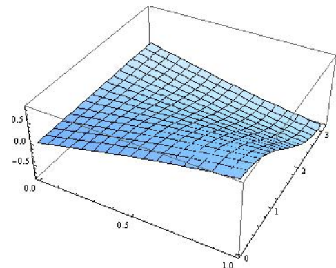
Fig. 5. The surface of \sigma_1(x, t)
