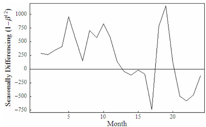
Fig. 3 Seasonally differencing 2 nd order with 12 months of DHF incidence in Northern Thailand from January 2003-December 2006
