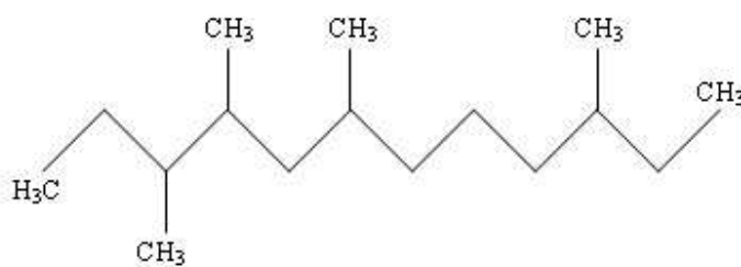
Fig. 1. (3, 4, 6, 10) - tetramethyldodecane
